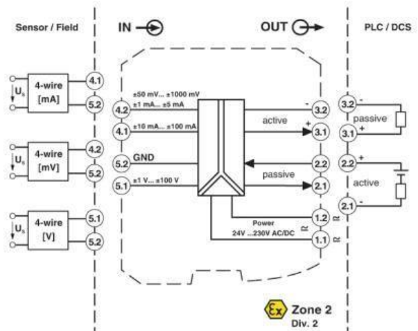
MACX MCR-UI-UI-UP-NC
