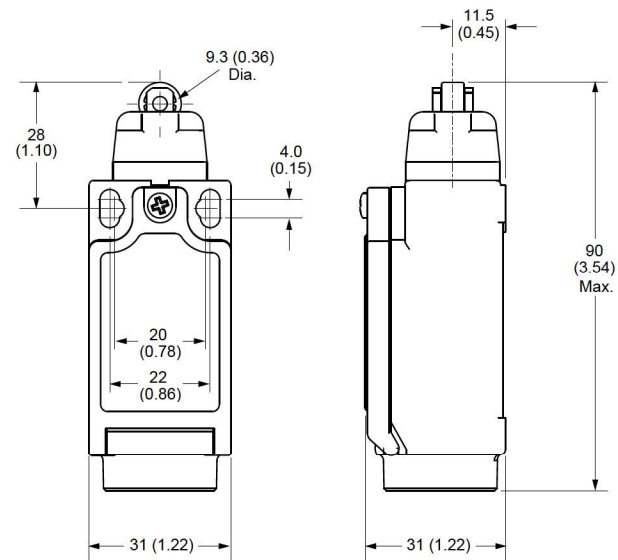
Roller Plunger
