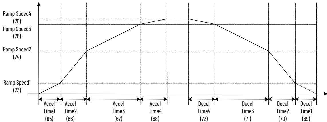
Figure 3 - Speed Reference: Linear Ramp
