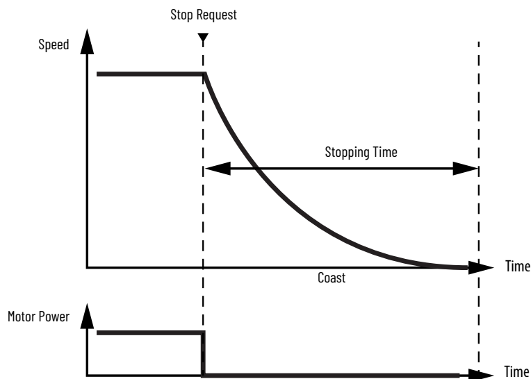
Figure 9 - Safe Torque Off Operation Chart
